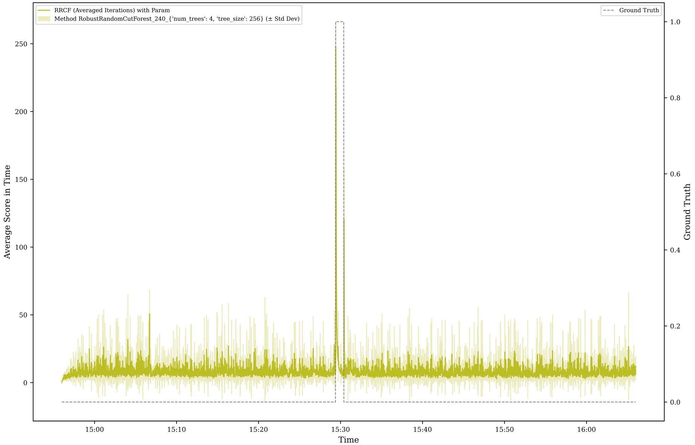
Method RRCF Score for Scenario A1
